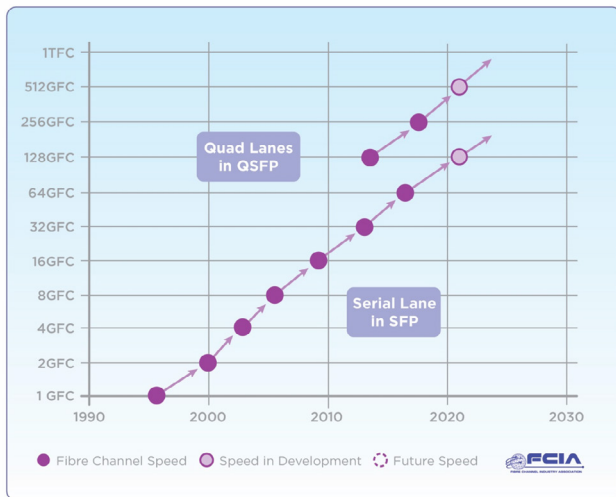
Figure 1: Fibre Channel Speeds
